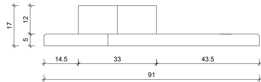
4 SECTION Scale - 1:1 @ A3
