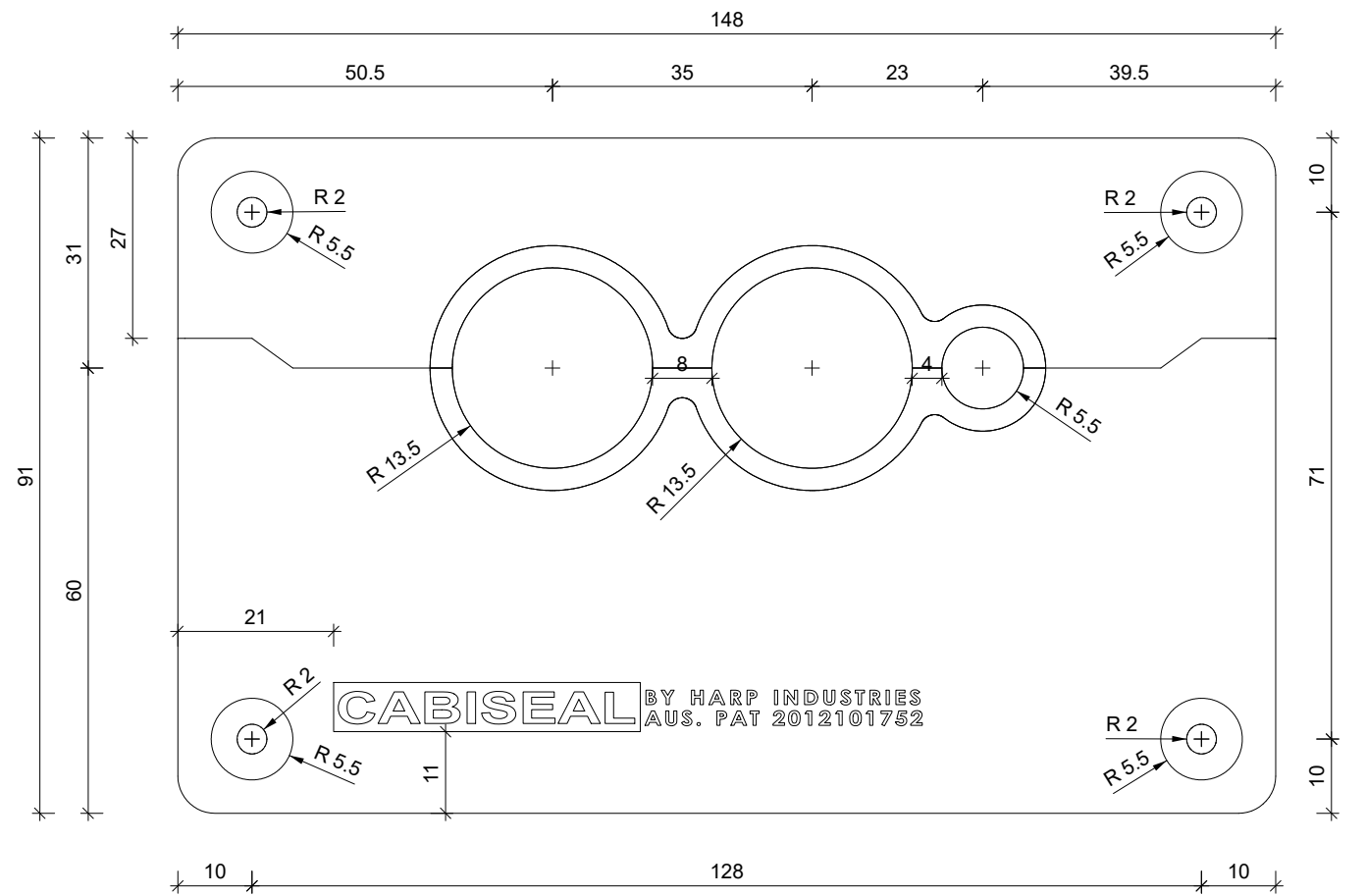
2 PLAN Scale - 1:1 @ A3
